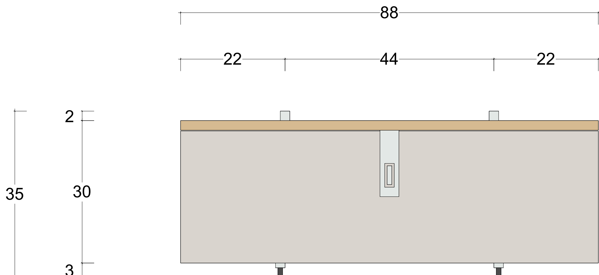
E1 LOCKERS - FRONT ELEVATION Scale: 1:5
