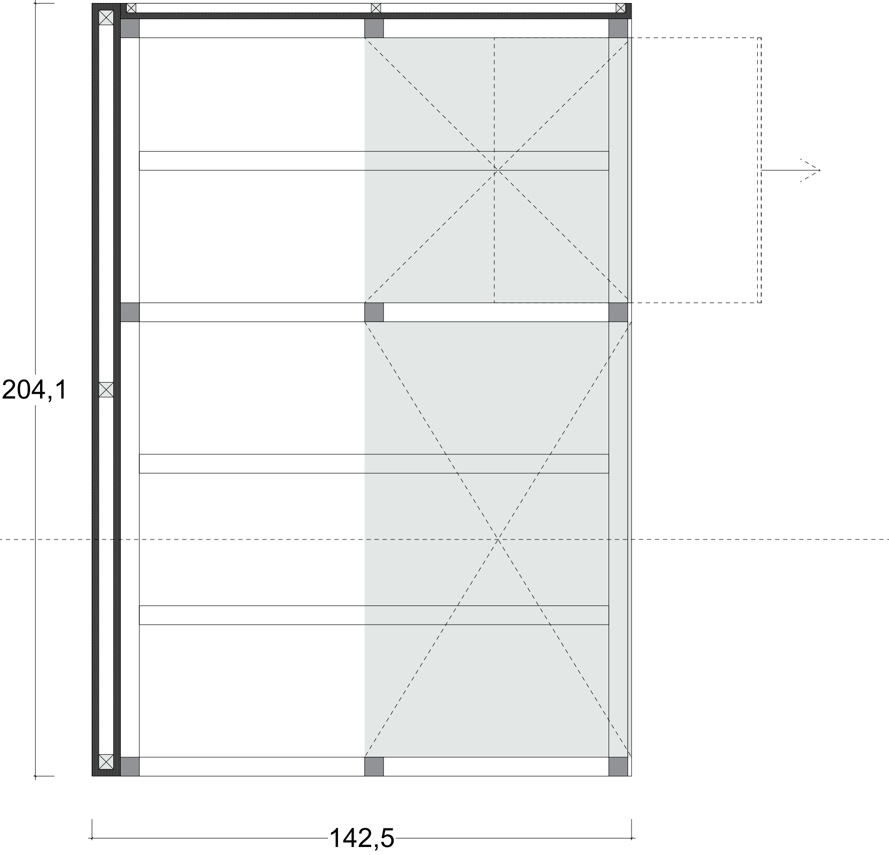
Top view
