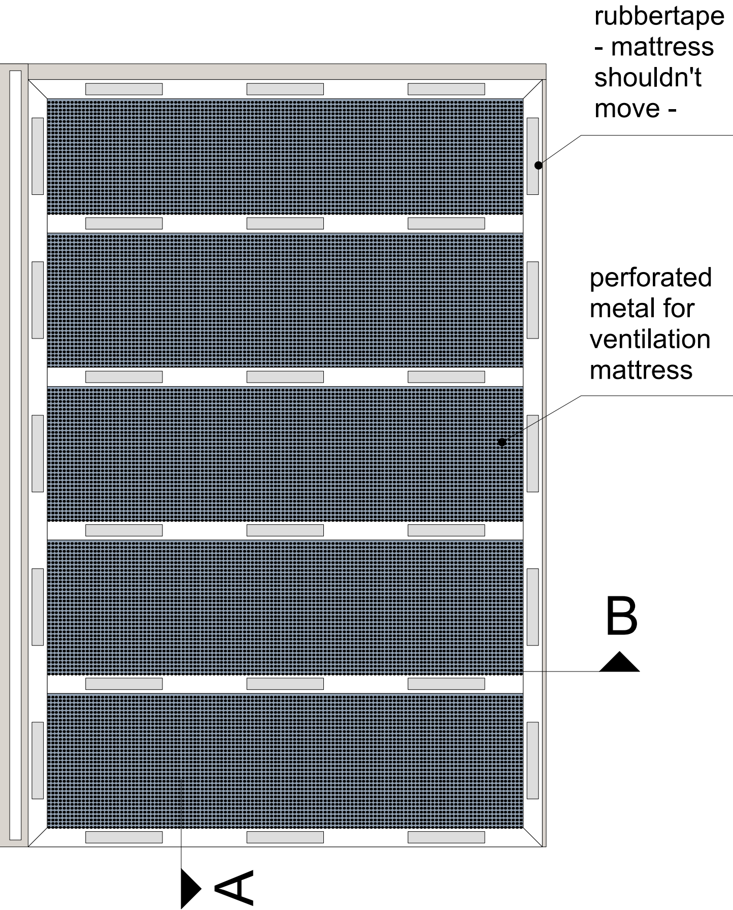
Top view
