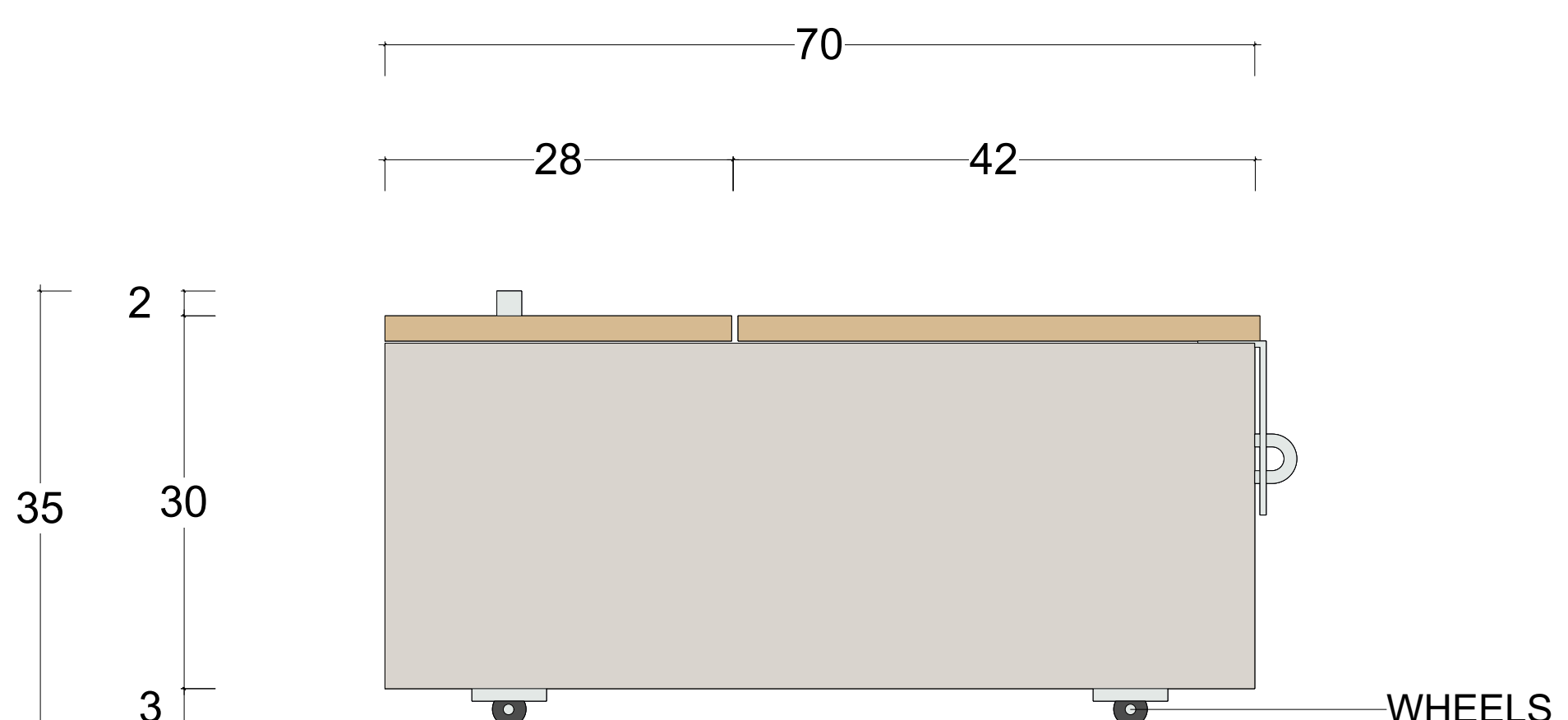
E2 LOCKERS - SIDE ELEVATION Scale: 1:5
