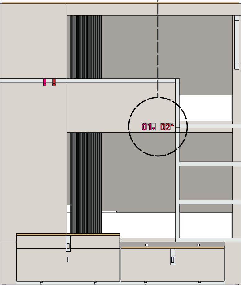
BUNKBED 2-A ELEVATIONS
