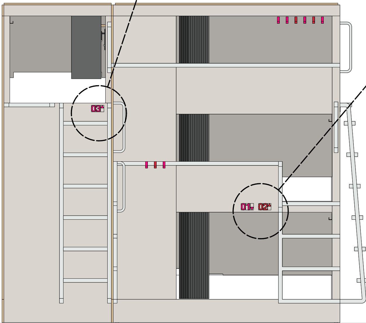
BUNKBED 3-B ELEVATIONS
