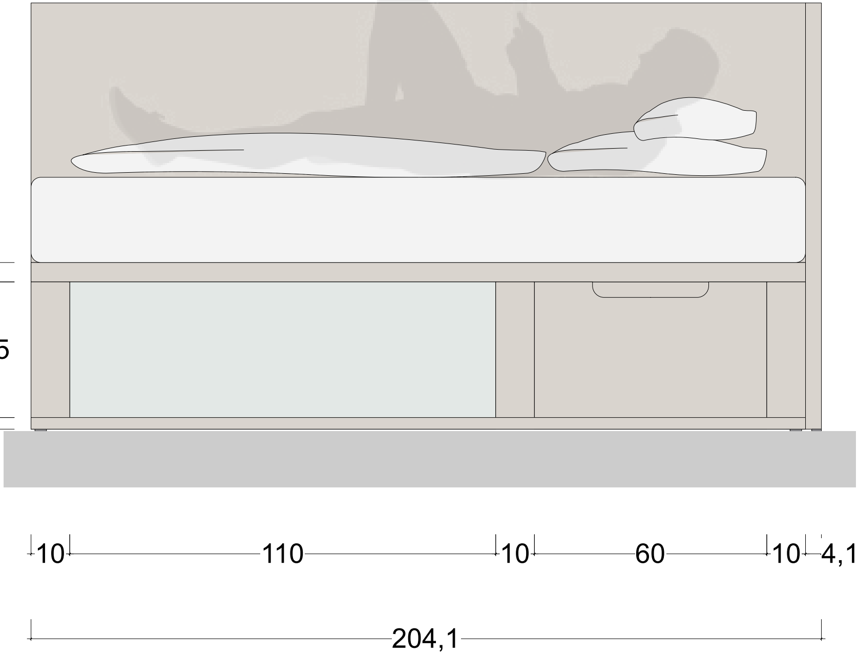
Side view
