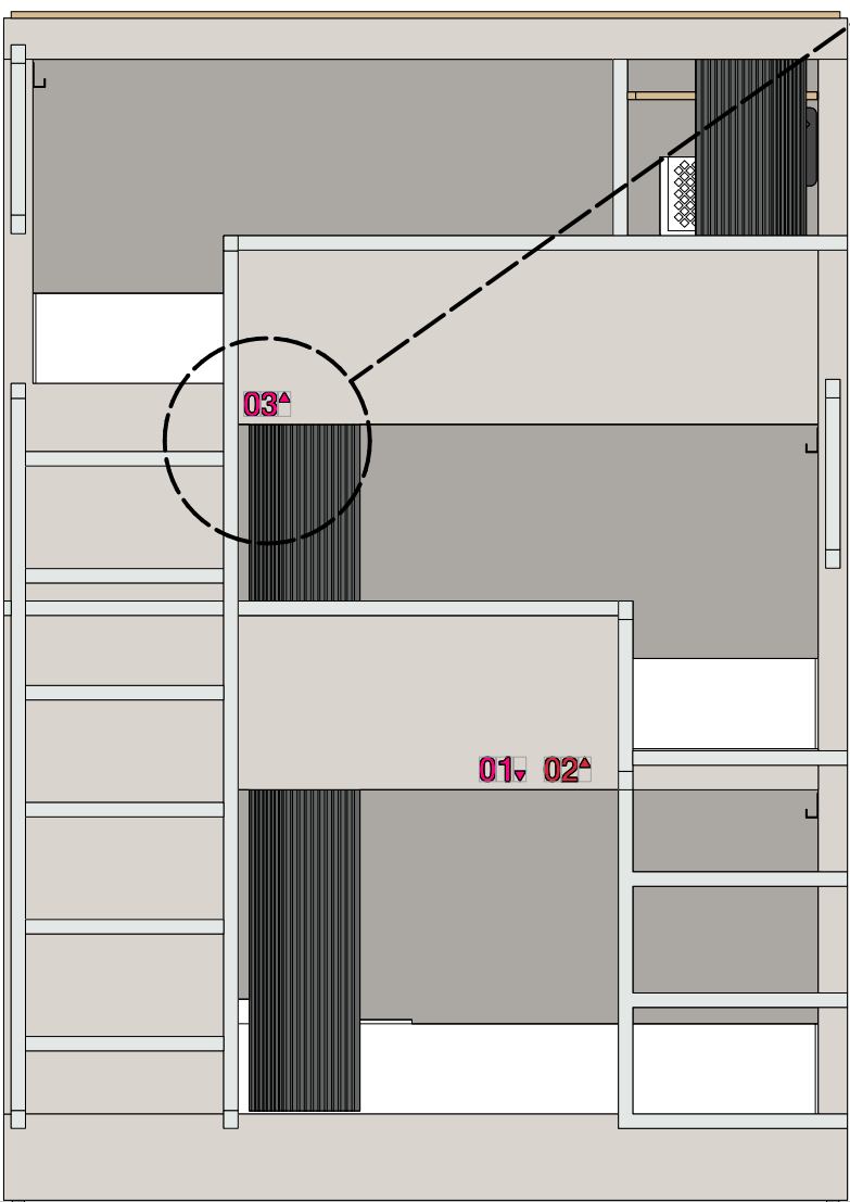
BUNKBED 3-A ELEVATIONS
